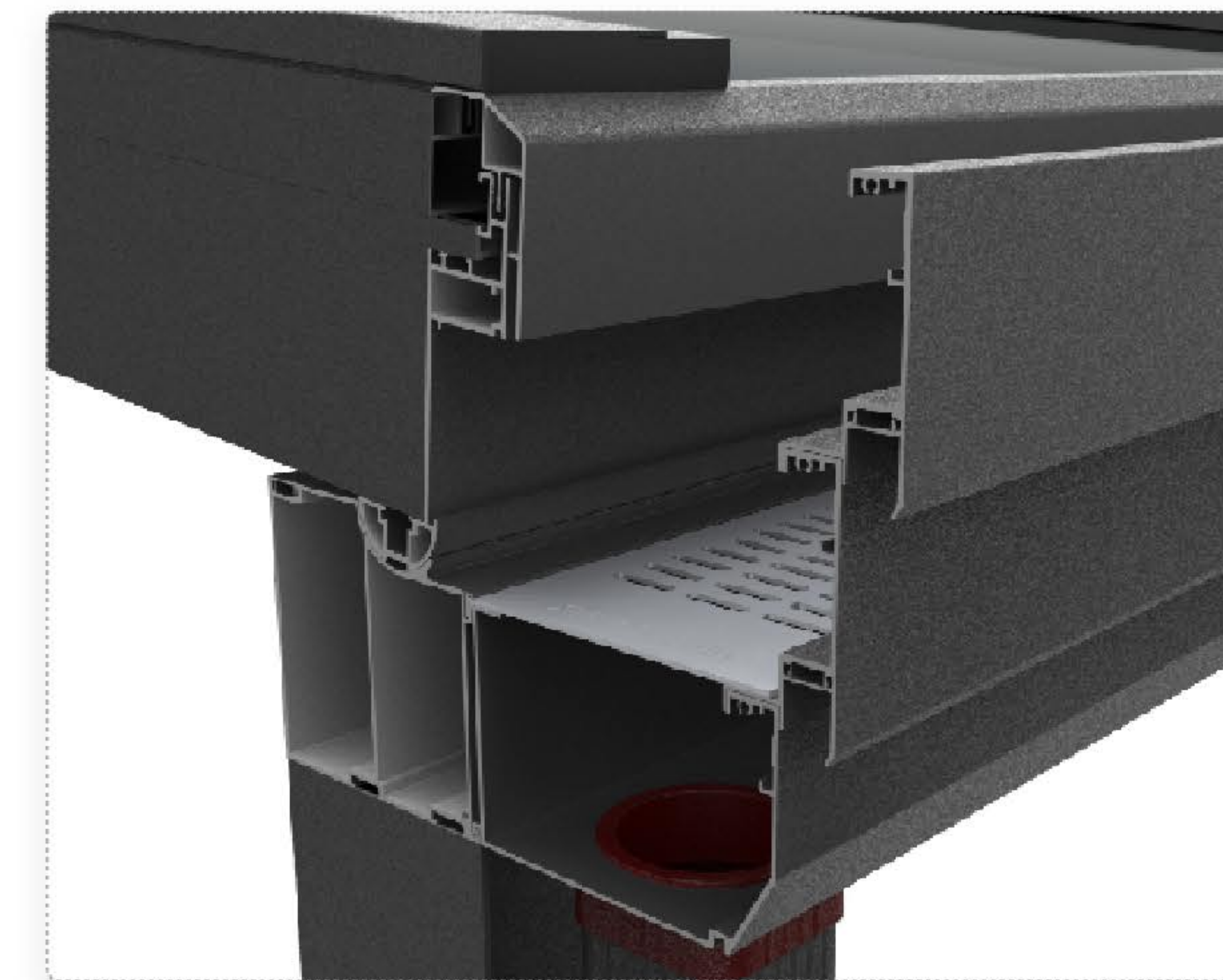
Drainage system
