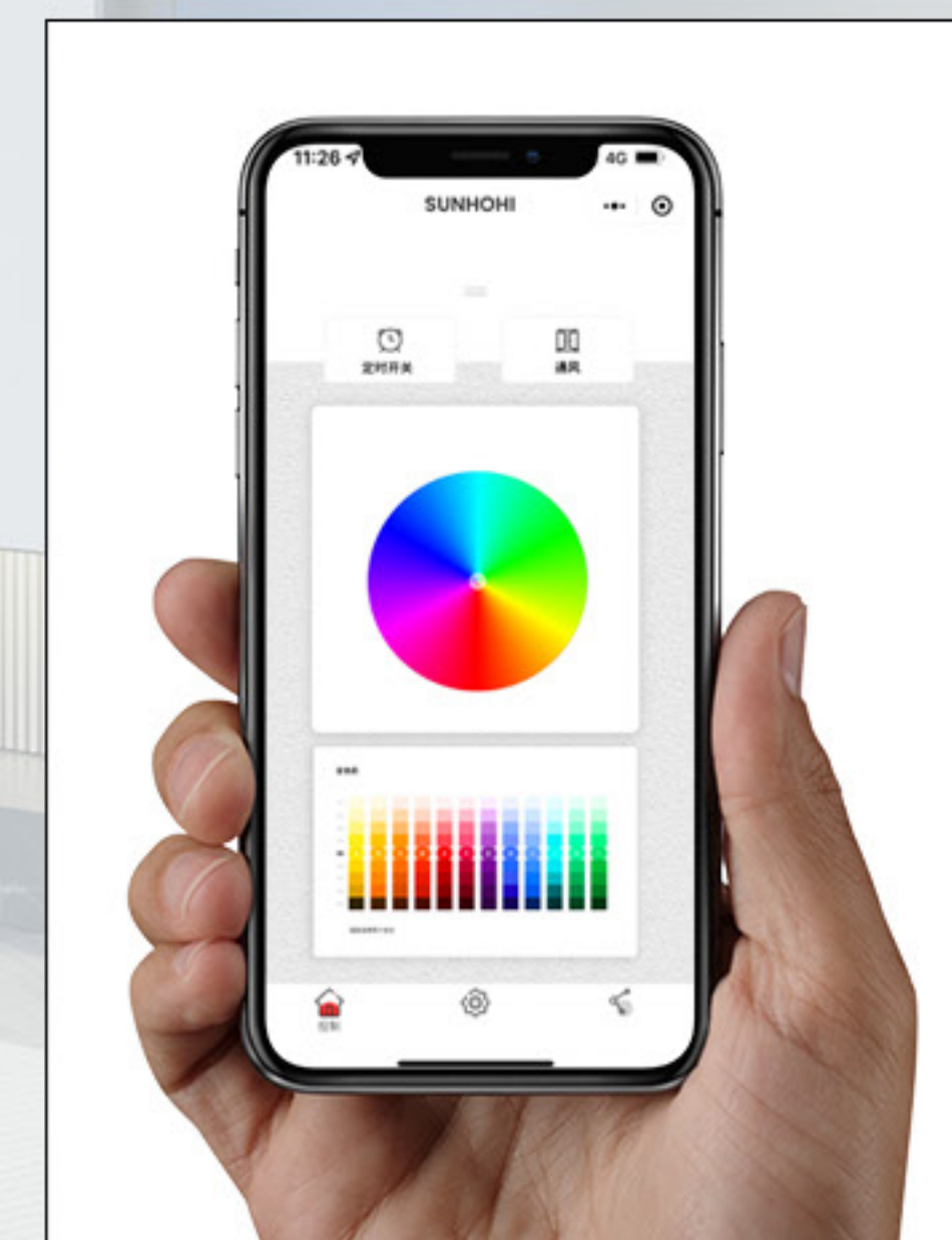
Mobile App
