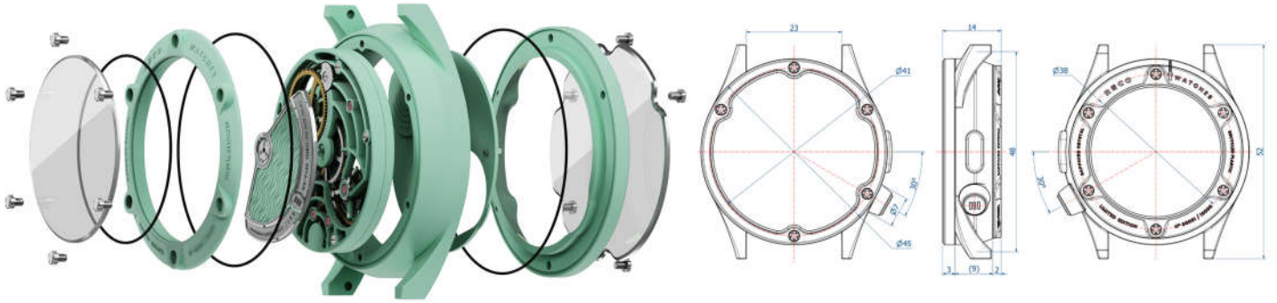
Exploded View
