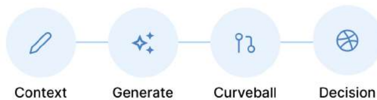
Figure 7. CICD Framework
